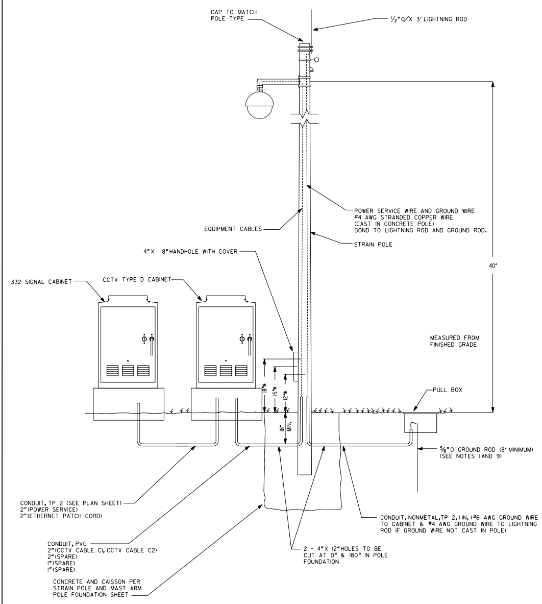
CCTV INSTALLATION ON SAME CORNER AS SIGNAL CABINET
