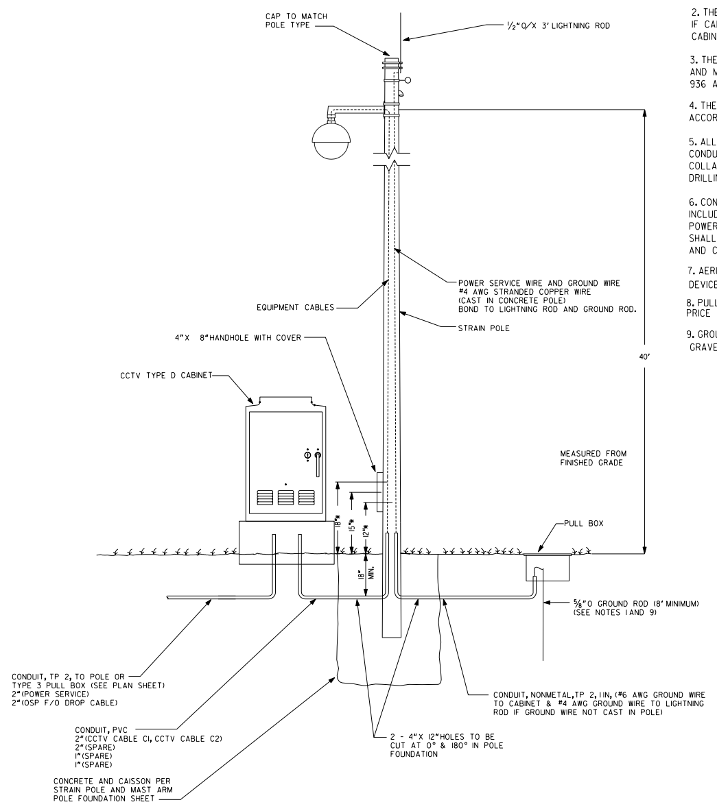
CCTV INSTALLATION ON DIFFERENT CORNER THAN SIGNAL CABINET
